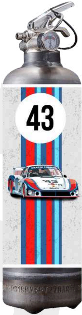
MARTINI 43 FD
